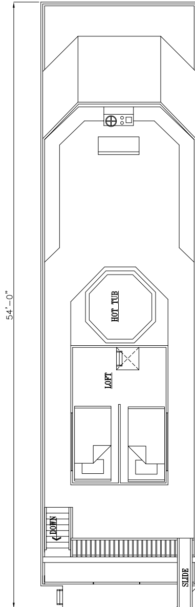
UPPER DECK PLAN
